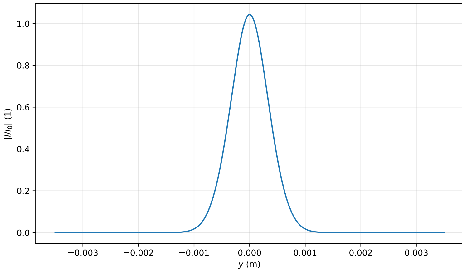
Intensity profile I(x=0, y, z=0.239)/I_0 , \text{Pin}=1.0\text{Pcr} , artificial time
